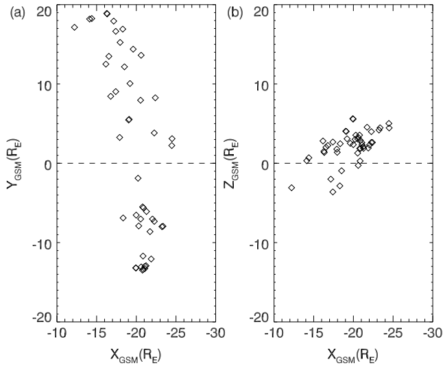
Figure 3. Location of the thin current sheet events observed by MMS in the (a) geocentric solar magnetospheric x - y plane and (b) geocentric solar magnetospheric x - z plane.
