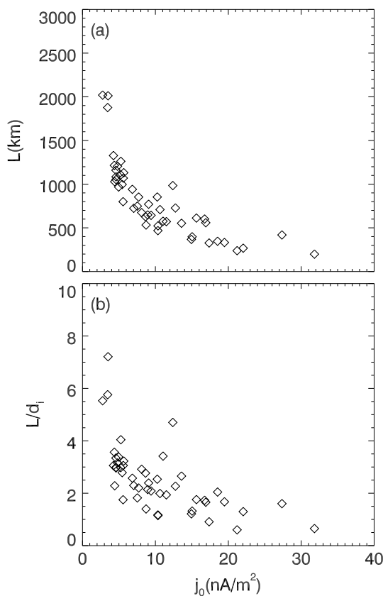
Figure A1. Current sheet thickness in the thin current sheet events in units of (a) kilometers and (b) local ion inertial length ( d_i , evaluated using peak ion density).
