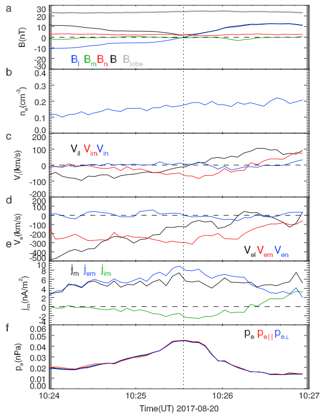
Figure 4. MMS1 observations of a thin current sheet from 10:24 to 10:27 UT on 20 August 2017. (a) Magnetic field, (b) electron density, (c) ion flow velocity, (d) electron flow velocity, (e) current density and electron and ion contributions in the \mathbf{m} direction, and (f) electron pressure (black), electron parallel pressure (red), and electron perpendicular pressure (blue).
