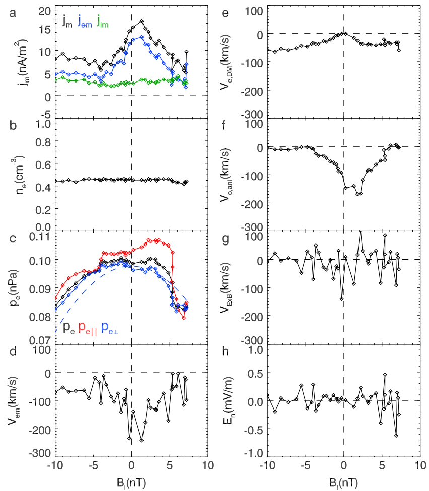
Figure 6. MMS1 observations of a thin current sheet from 16:56 to 16:59 on 18 August 2017. Same format as Figure 5.
