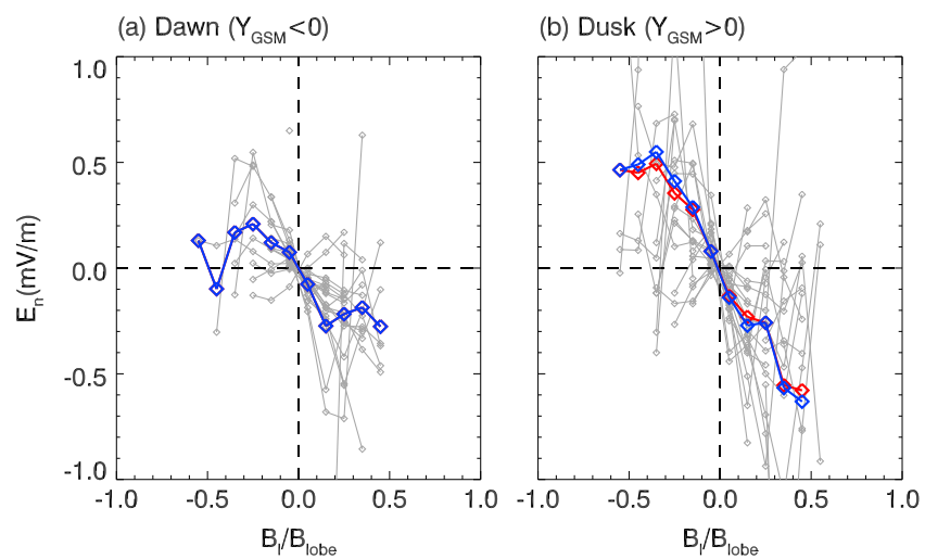
Figure 7. (a, b) Statistics and dawn-dusk asymmetry from MMS measurements. The magnetic field B_l is normalized to the magnitude of the lobe magnetic field B_{lobe} (we use plasma pressure, p_p = k_B(n_e T_e + n_i T_i) to calculate B_{lobe} from the current sheet pressure balance, B_{lobe} = (B_x^2 + B_y^2 + 2\mu_0 p_p)^{1/2} ). Each gray curve represents a single event. The red curve denotes the average of all the events, and the blue curves denote the average of the events in which \mathbf{E} \times \mathbf{B} drift dominates the electron velocity (i.e., the strong anisotropy events are excluded).
