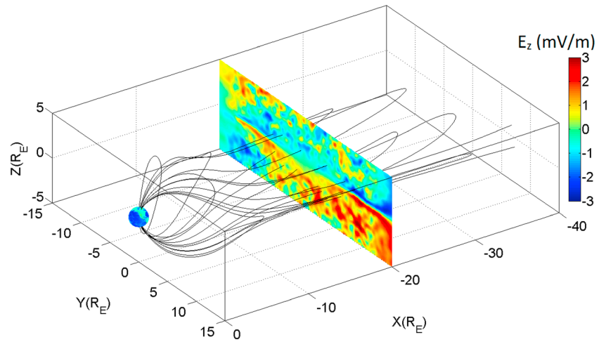
Figure 1. Global hybrid simulation result of Auburn Global hybrId CodE in 3-D showing the configuration of magnetic field lines and the contour of Hall electric field E_z at x = -20 R_E at t = 1, 144 s. The simulation uses a pure southward interplanetary magnetic field, -10 nT, and a steady solar wind speed in the x direction, -700 km/s. The structure of the magnetotail (characterized by stretched field lines) forms self-consistently via interaction between the interplanetary magnetic field/solar wind and the geomagnetic field. The Hall electric field E_z forms in the magnetotail thin current sheet. For more details of the simulation model, see Lin et al. (2014, 2017).
