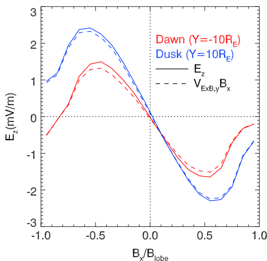
Figure 2. Profiles of the Hall electric field E_z from Auburn Global hybrId CodE in 3-D at x = -20 R_E on the duskside ( y = 10 R_E ) and the dawnside ( y = -10 R_E ) at t = 1, 144 s. The dashed curves represent the electric field calculate using E_z = V_E \times B, y B_x , where V_E \times B, y = (E_z B_x - E_x B_z) / B^2 . The magnetic field B_x indicates the distance to the center of the current sheet, and it is normalized to the magnitude of the lobe magnetic field B_{lobe} (we use plasma pressure at the current sheet center to calculate B_{lobe} from the pressure balance).
