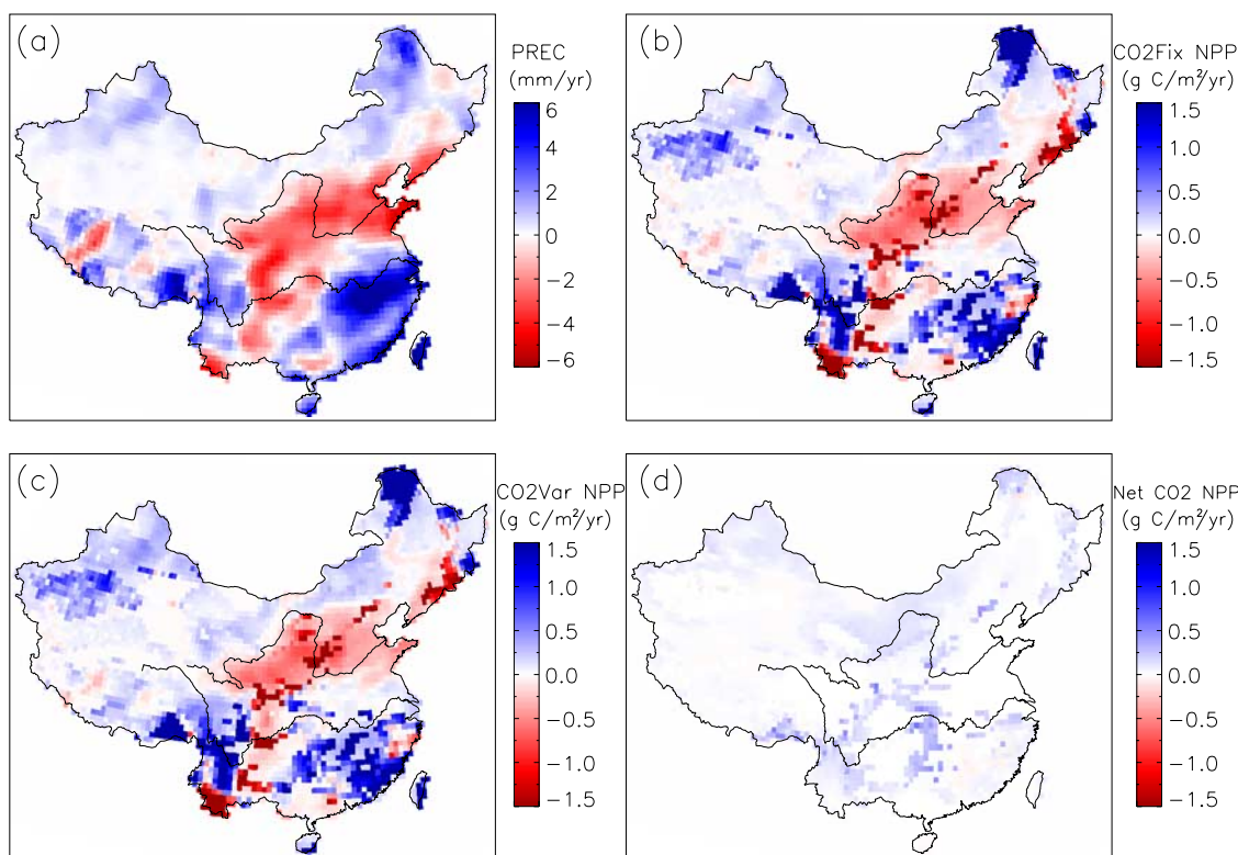
Figure 2. The 0.5° spatial trends of (a) observed precipitation (PREC) and NPP estimated by Biome-BGC during 1961–2000 driven by (b) fixed CO 2 (at 1961 level) and variable meteorology data (CO2Fix NPP) and (c) variable CO 2 concentration and meteorology (CO2Var NPP). (d) Net CO 2 fertilization effects (Net CO 2 NPP); net CO 2 effects are calculated as the difference between CO2Var and CO2Fix.
