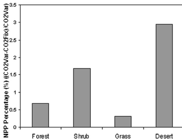
Figure 8. Percentage of net CO 2 fertilization effects on NPP (CO 2 Var – CO 2 Fix) as compared to the NPP average from CO 2 Var.
